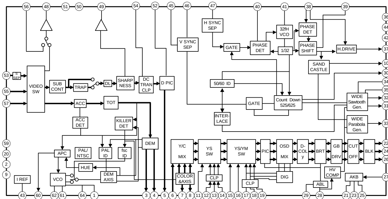
A BOARD IC301 CXA2000Q-TL
