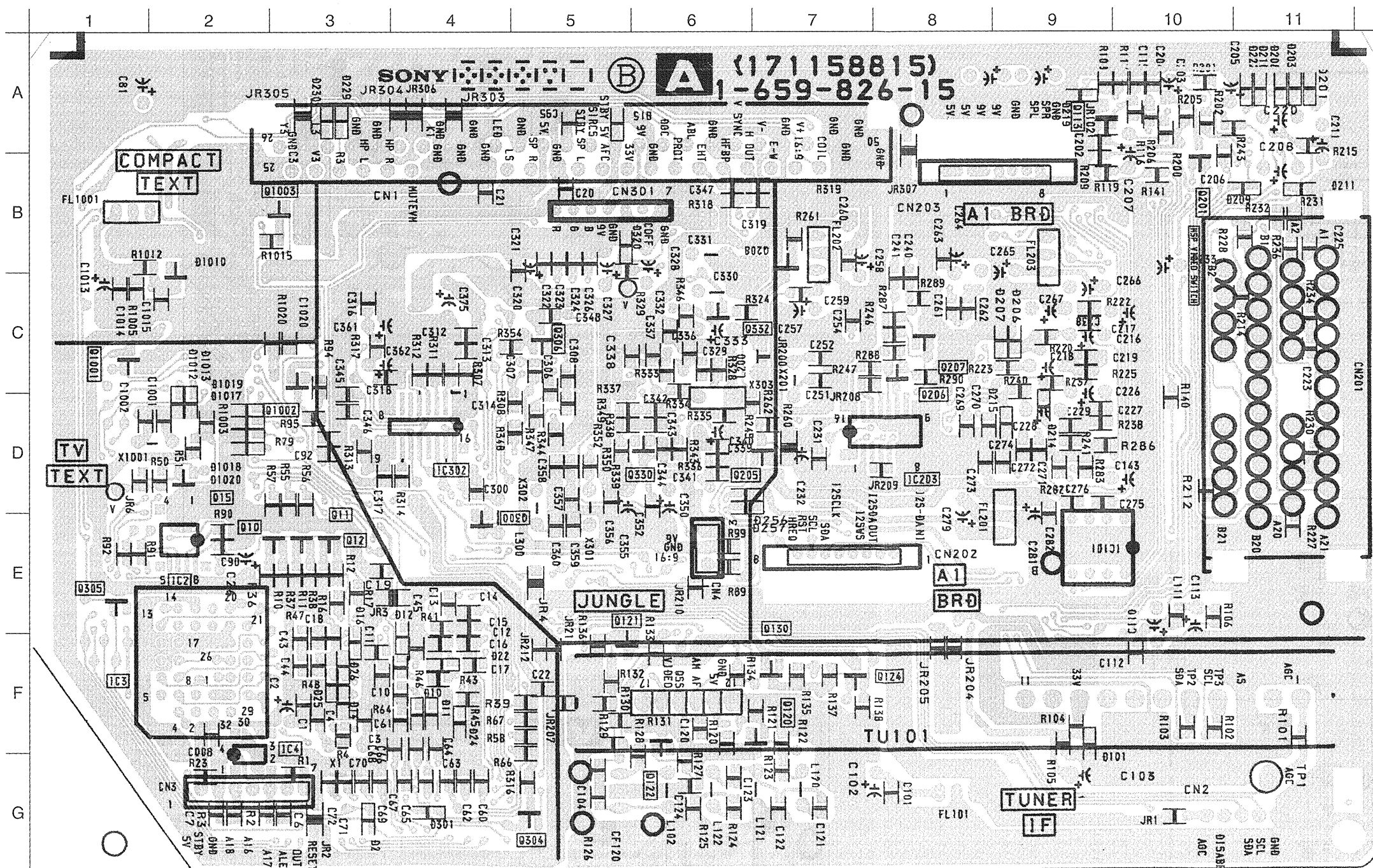
A Board &lt; Conductor Side &gt;
