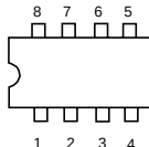
LM393P M5216P TDA2822M \mu PC393C
