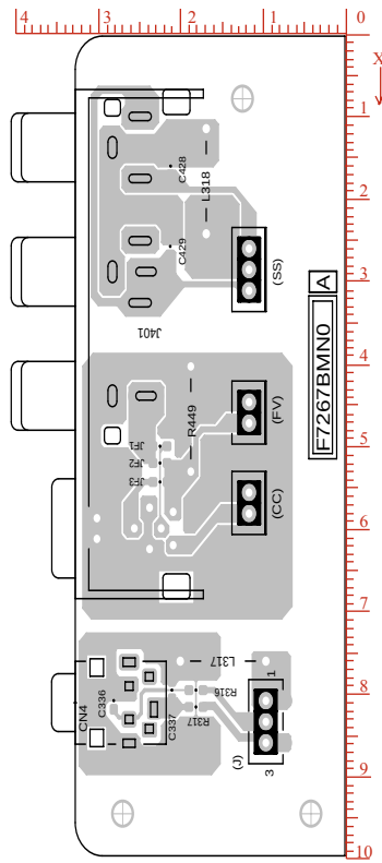
Copper Side
