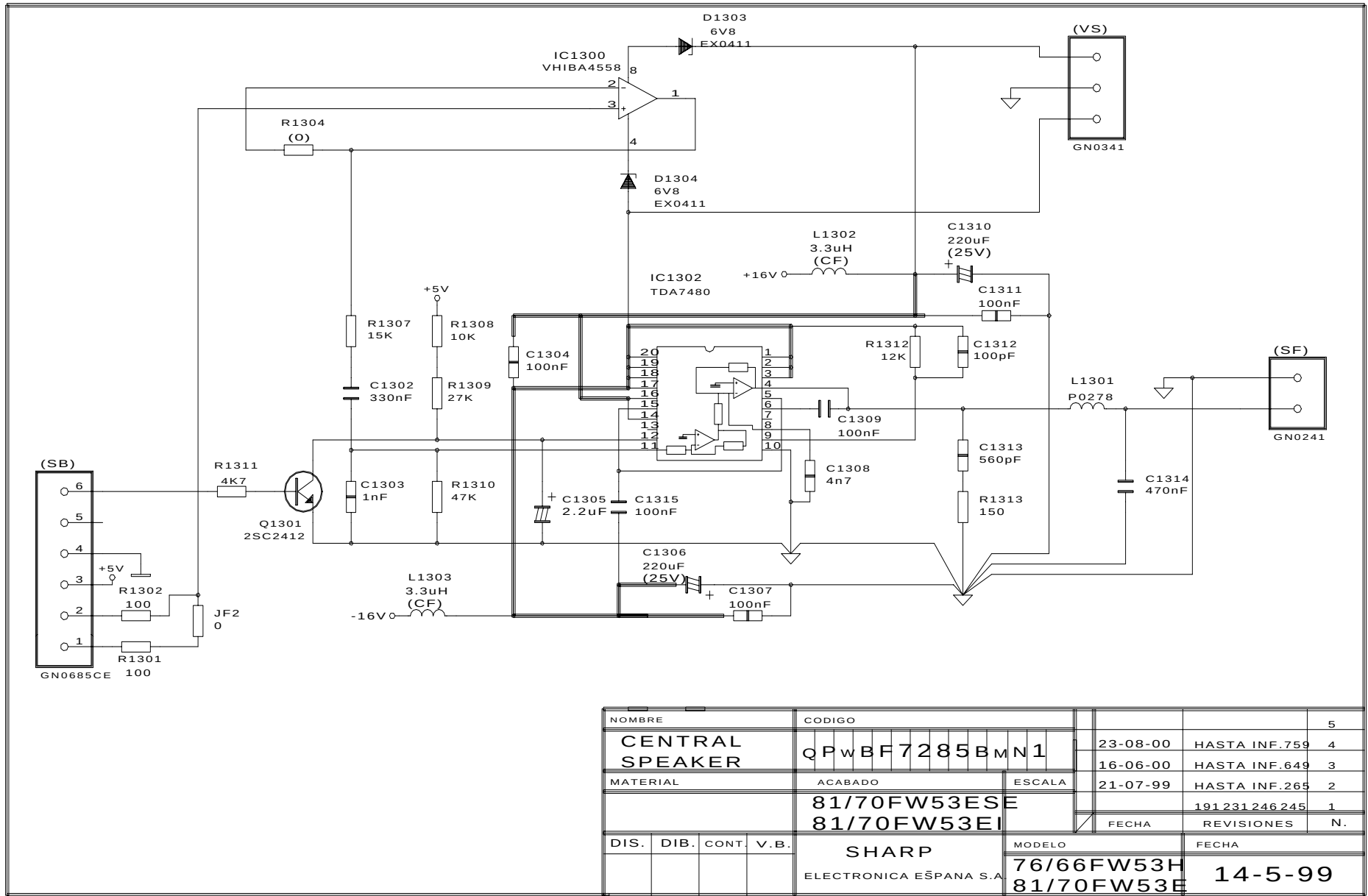
SCHEMATIC DIAGRAM OF CENTRAL SPEAKER UNIT (F7285N1A), 00 Version.
