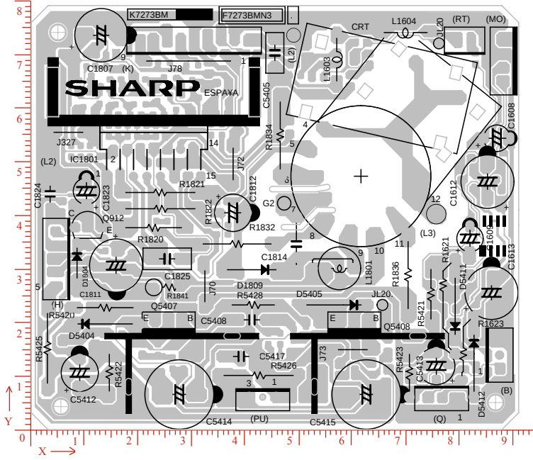
Copper Side
