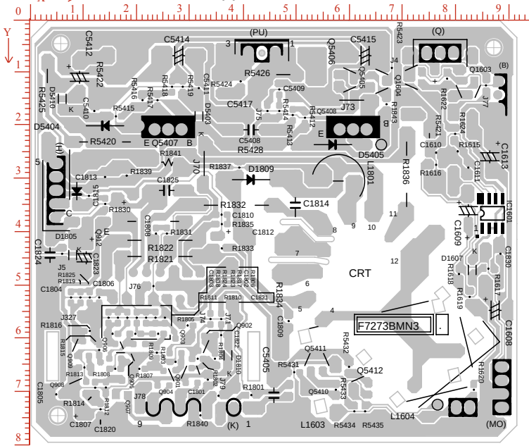
Copper Side
