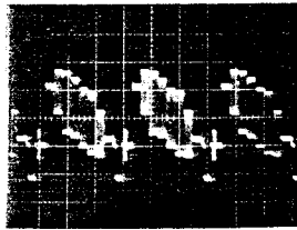
Point : A 1Div=20uS 1Div=0.5V
