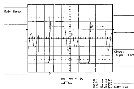
Q903 collector
