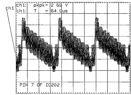
Pin 7 of IC202
