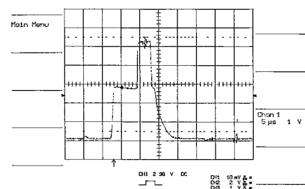
IC501 Pin 41
